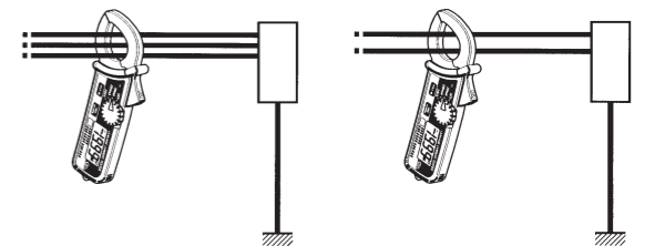
Three-phase, 3-wire systems Single-phase, 2-wire systems In a 4-wire system, clamp onto all 4 wires. In a 3-wire system, clamp onto all 3 wires.
