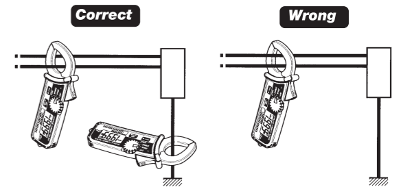
Fig. 1 Normal Measurement
